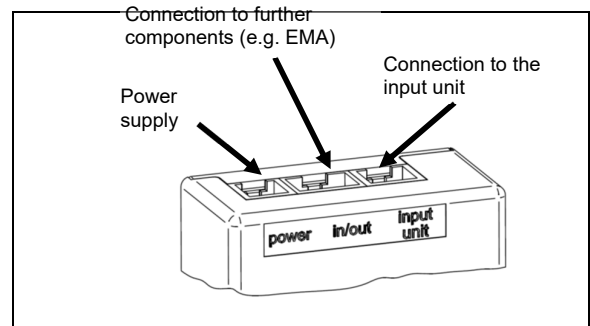
Figure 4: Connections at the lock housing
