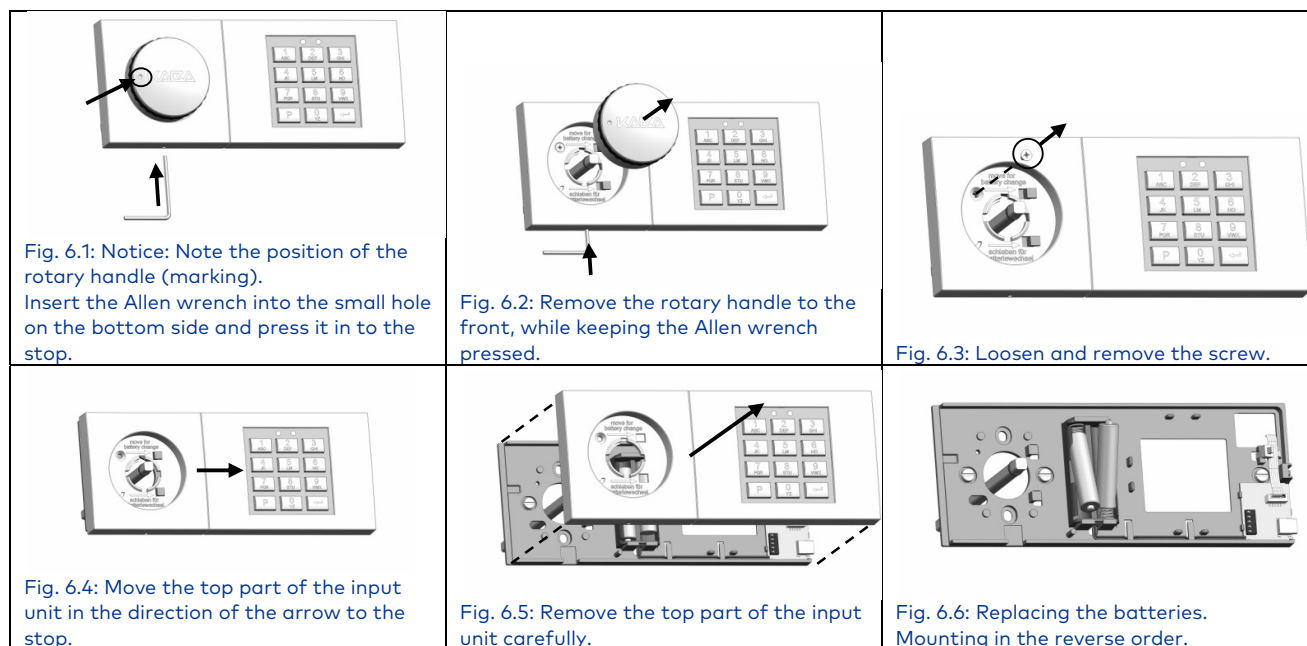
Figure 6: Battery replacement
